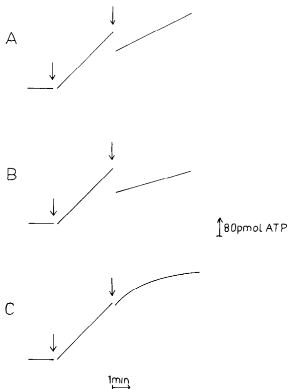
Fig.4. Time course of ATP synthesis in a suspension of PPase,ATPase liposomes; 50 \mu l liposomes were suspended in a medium described in fig.3. At the first arrow in A, the liposomes were added; at the second arrow 10 \mu l 10 mM DCCD was added. At the first arrow in B, liposomes were added; at the second arrow 50 \mu l oligomycin (2 mg/ml) was added. At the first arrow in C, liposomes were added; at the second arrow 4 \mu l efrapeptin (1 mg/ml) was added.
