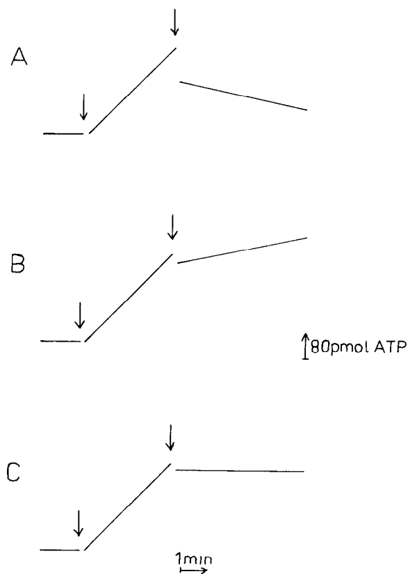
Fig.5. Time course of ATP synthesis in a suspension of PPase,ATPase liposomes; 50 \mu l liposomes were suspended in a medium described in fig.3. At the first arrow in A, the liposomes were added; at the second arrow 30 \mu l 0.4 NaF was added. At the first arrow in B, liposomes were added; at the second arrow 30 \mu l 20 mM MDP was added. At the first arrow in C, liposomes were added; at the second arrow 30 \mu l 20 mM IDP was added.
