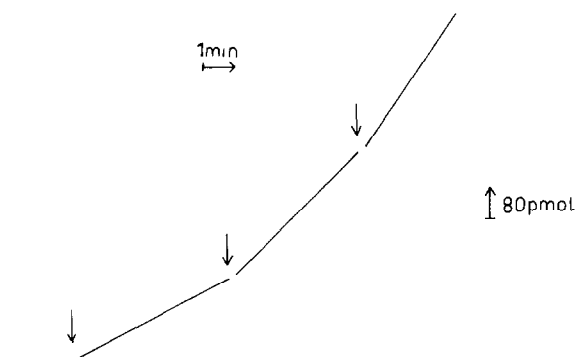
Fig. 3. Time course of ATP synthesis as a function of the amount of liposomes added; (—) 25 \mu l liposomes added to the same medium as in fig. 1 except that 50 \mu l 10 mM sodium pyrophosphate was present.
