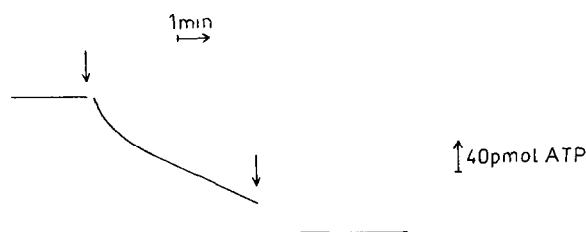
Fig. 2. Time course of ATP hydrolysis in a suspension of PPase, ATPase liposomes; 50 \mu l liposomes were suspended in the same medium as in fig. 1 except that no sodium pyrophosphate was added. At the first arrow 50 \mu l liposomes was added. At the second arrow 50 \mu l oligomycin (2 mg/ml) was added.
